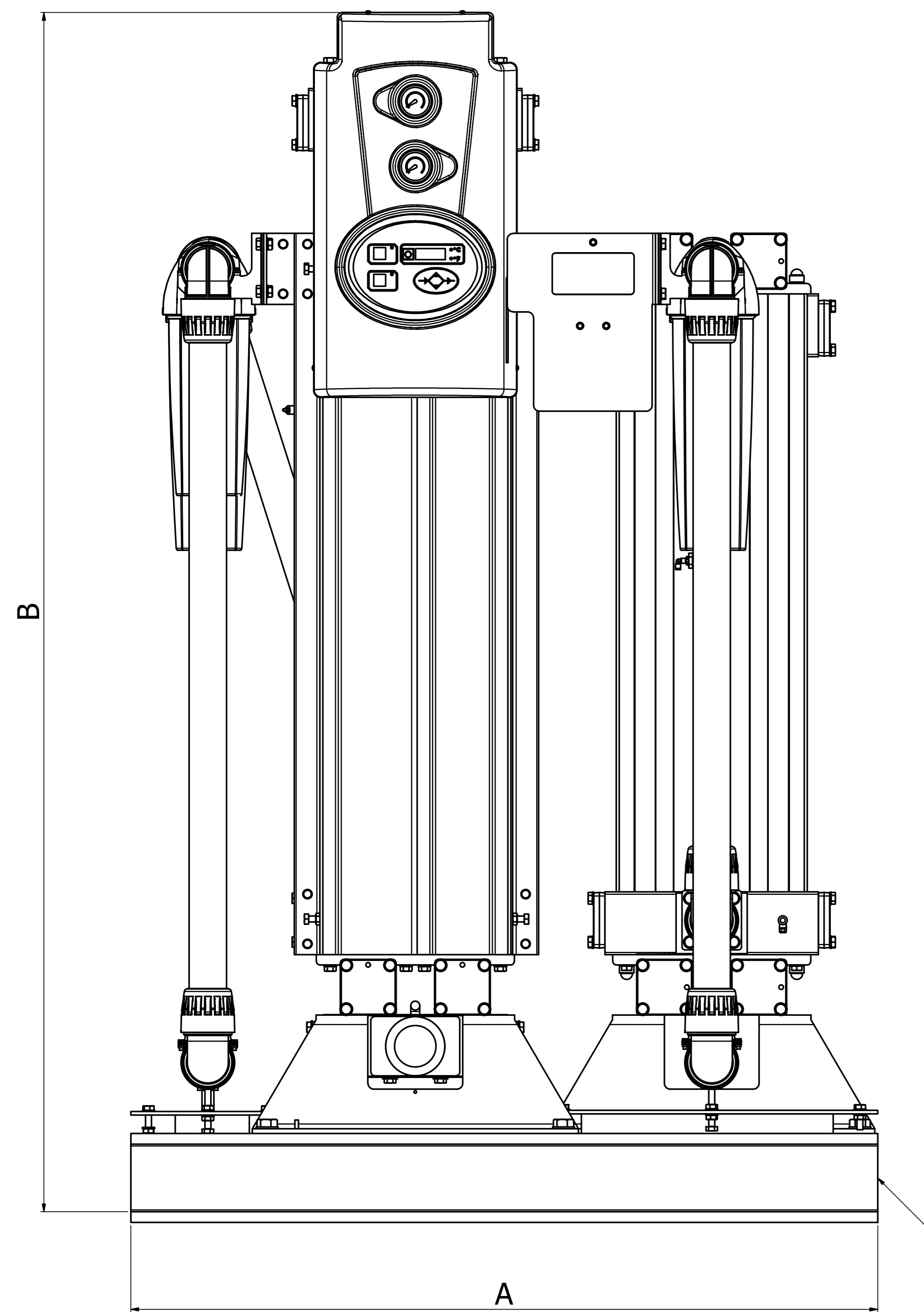
FRONT ELEVATION
